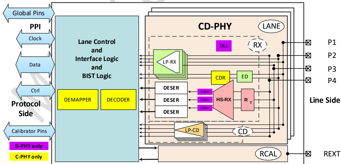
Figure 3-1: MIPI CD-PHY Block Diagram
