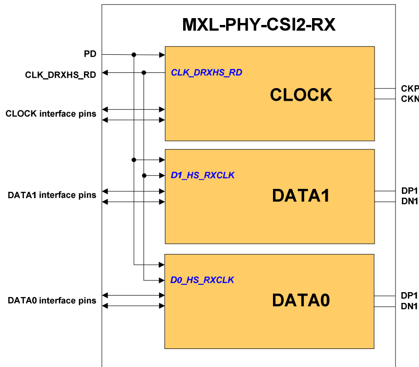
Figure 1 – PHY Block Diagram
