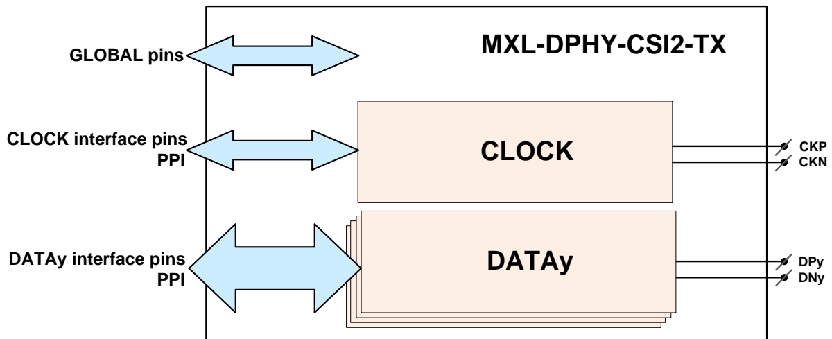
Figure 1: MIPI D-PHY CSI-2-TX Block Diagram
