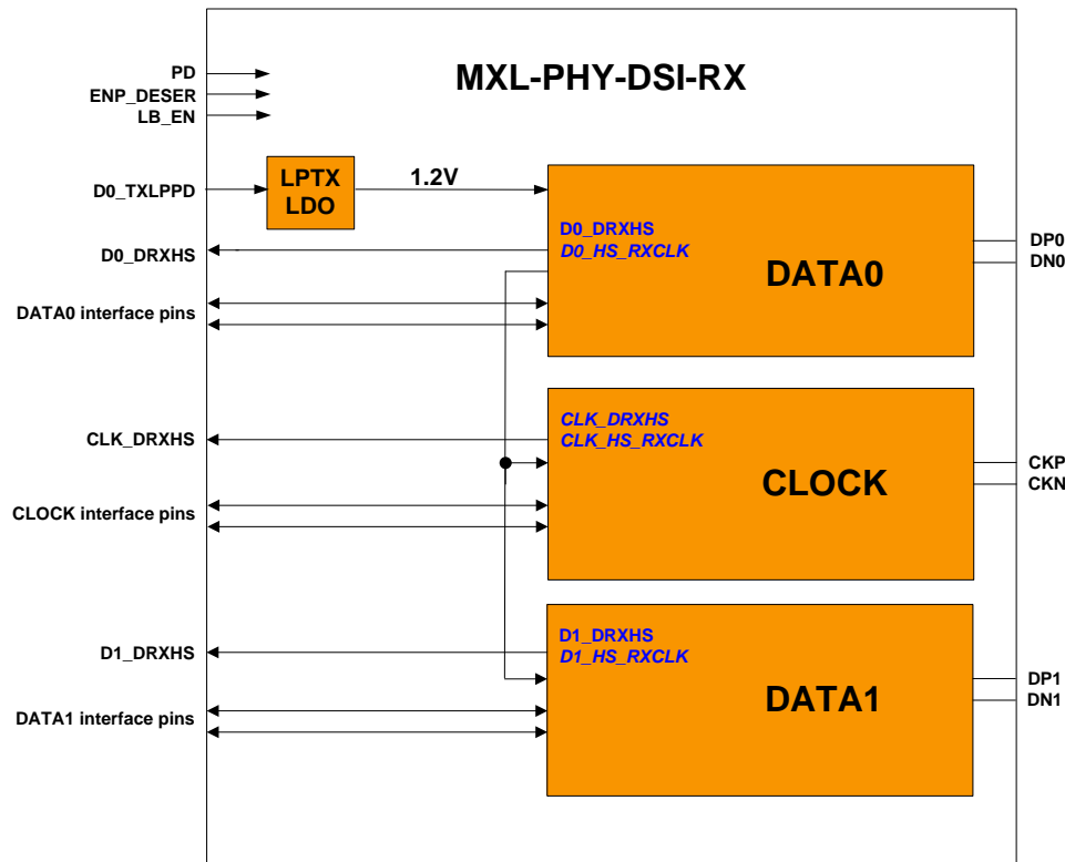
Figure 1 – PHY Block Diagram
