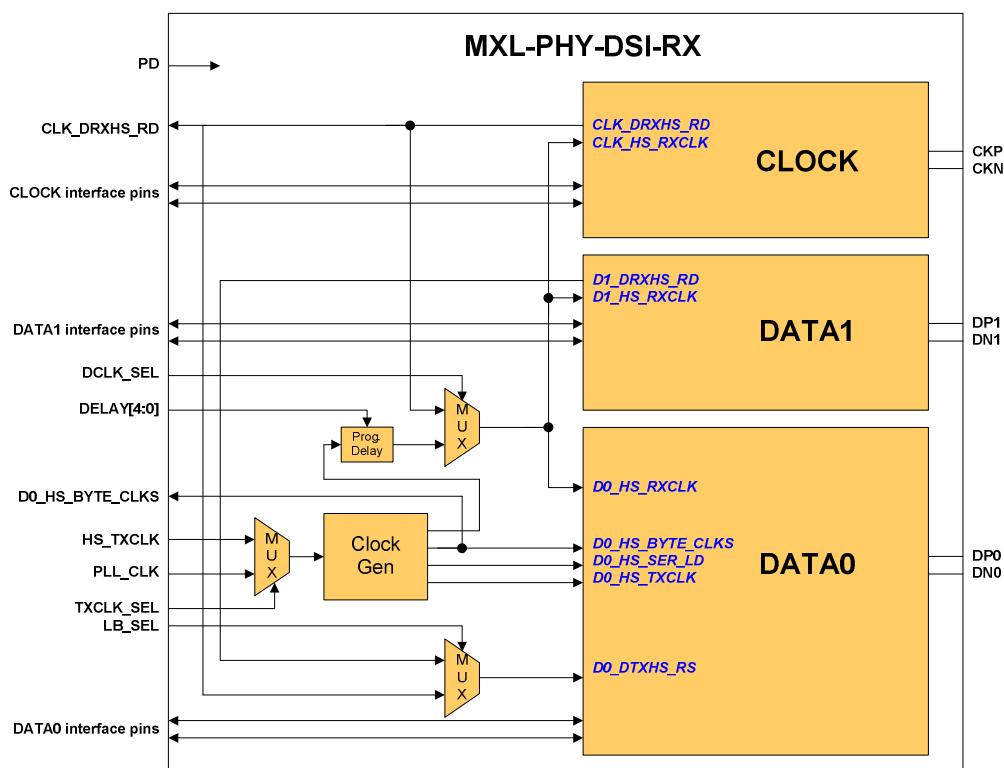
Figure 1 – PHY Block Diagram
